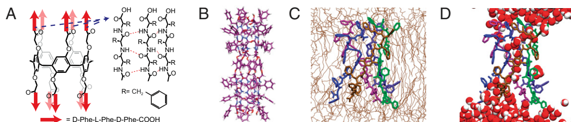
Fig. 1. Structure of the peptide-appended pillar[5]arene (PAP) channel. (A) The PAP channel ( C_{325}H_{320}N_{30}O_{60} ) forms a pentameric tubular structure through intramolecular hydrogen bonding between adjacent alternating D-D phenylalanine chains (D-Phe-L-Phe-D-Phe-COOH). (B) Molecular modeling (Gaussian09, semiempirical, PM6) of the PAP channel shows that the benzyl rings of the phenylalanine side chains extend outward from the channel walls (C, purple; H, white; O, red; N, blue). (C and D) MD simulation of the PAP channel in a POPC bilayer revealed its interactions with the surrounding lipids. The five chain-like units of the channel are colored purple, blue, ochre, green, and violet, with hydrogen atoms omitted. In C, the POPC lipids are represented by thin tan lines; in D, water is shown as red (oxygen) and white (hydrogen) van der Waals spheres.
